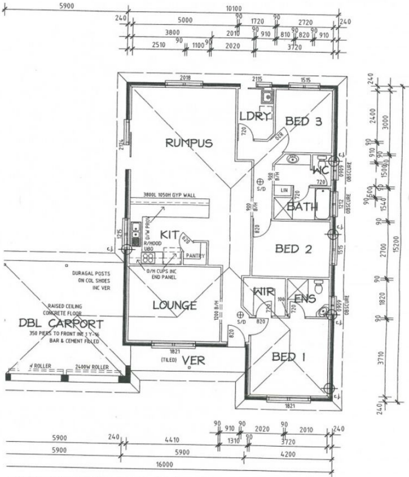
OLD SERIES 155 (E) FLOOR PLAN
