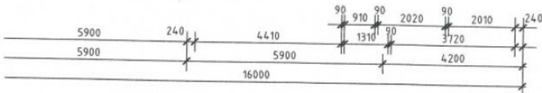
OLD SERIES 155 (E) FLOOR PLAN
